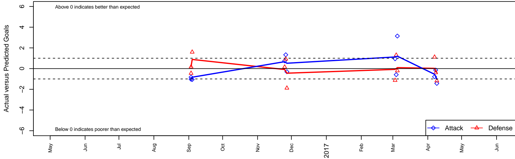
CCV Stars Black B00 Dots are actual minus expected GF (blue circles) and GA (red triangles). Blue line is smoothed change in attack strength. Red is smoothed change in defense strength.
